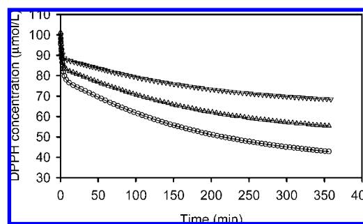
Figure 5. Time evolution of the concentration curves of DPPH* in methanol during its reduction by three different initial concentrations of protocatechuic acid. See Table 3 for the initial concentrations of DPPH* and protocatechuic acid.
