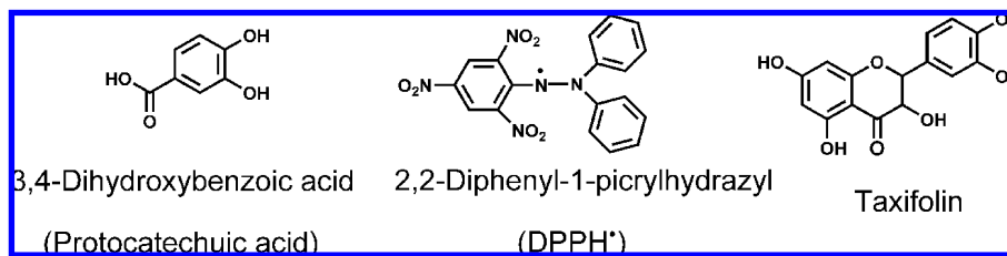
Figure 1. Chemical structures of the experimental and referenced compounds.
