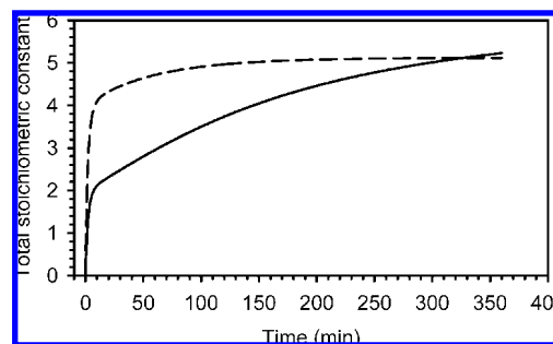
Figure 6. Time evolution of the total stoichiometric constant ( \sigma_t ) from protocatechuic acid methyl ester (---, y_0 = 103.261 \mu\text{mol/L} , a_0 = 11.780 \mu\text{mol/L} ) and protocatechuic acid (—, y_0 = 100.334 \mu\text{mol/L} , a_0 = 11.027 \mu\text{mol/L} ) during the reduction of DPPH* in methanol.
